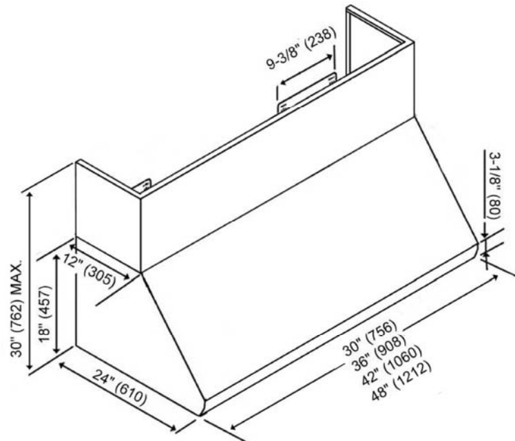
***Hood-Mounting Bracket
