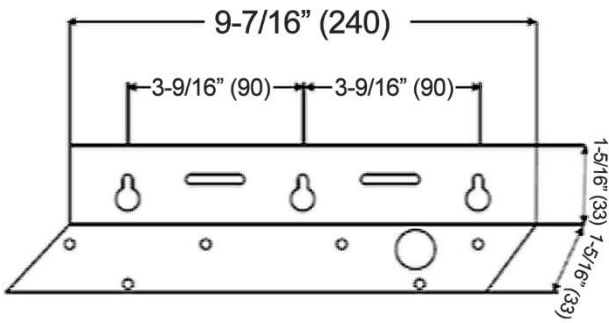
***Hood-Mounting Bracket
