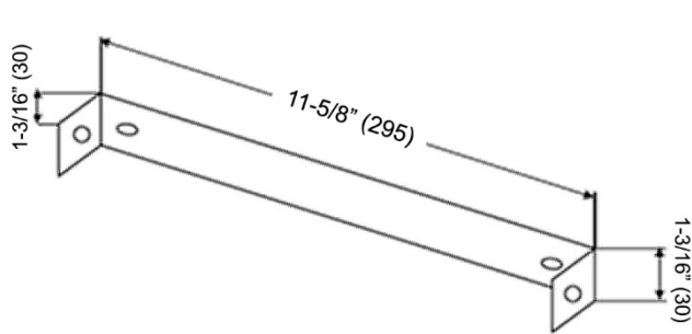
***Duct Cover-Mounting Bracket
