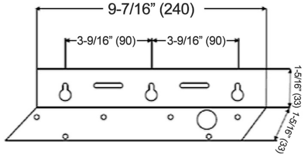
***Hood-Mounting Bracket
