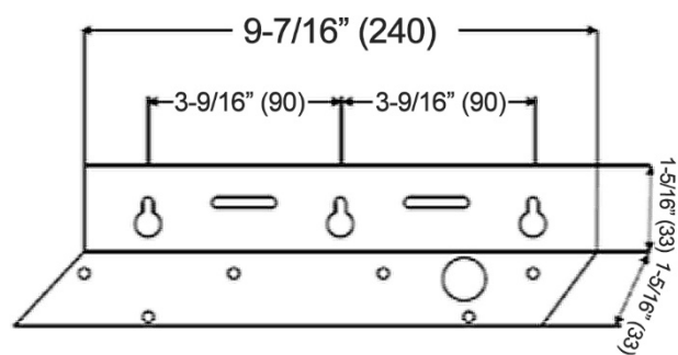
***Hood-Mounting Bracket
