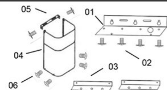
Duct Cover (Only for CH22 SQB-WM-1 Series)
