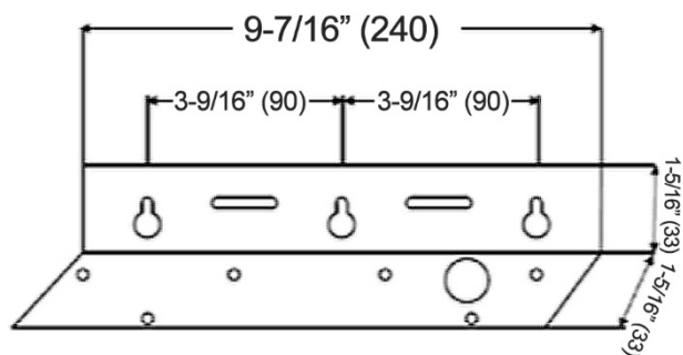
***Hood-Mounting Bracket
